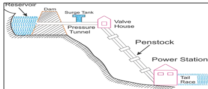
Figure 01 Layout
